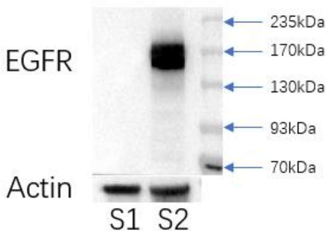
Figure 2 | The protein expression levels of Human EGFR(D770_N771insSVD-T790M) in the H_EGFR(D770_N771insSVD-T790M) BAF3 Cell Line (Cat. GM-C29682) were determined by Western blotting (WB).
